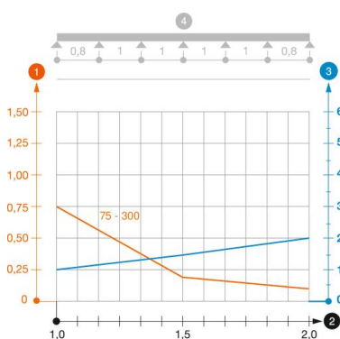
Load diagram, cable ladder, type SL42 ALU
